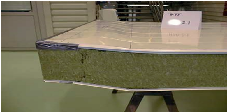
Figure 35: Failure of a specimen in a support reaction test (the final failure was shear)
