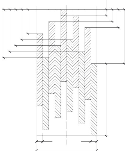
Figure 46: Example of the arrangement of MW lamellas
