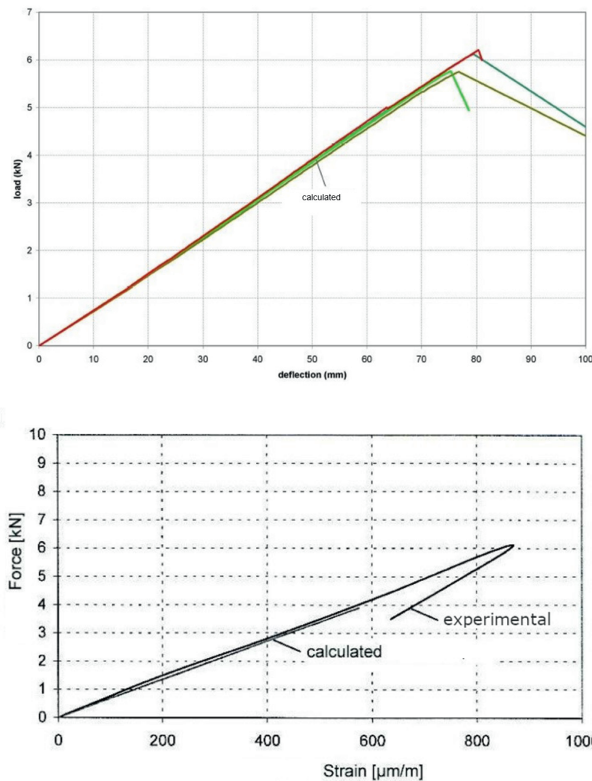
Figure 50: Load/deflection diagram and load/strain diagram
