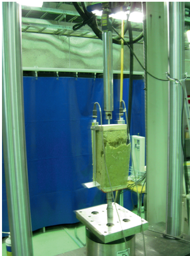
Figure 14: Cross-panel tensile test - measurement of the movement directly from specimen
