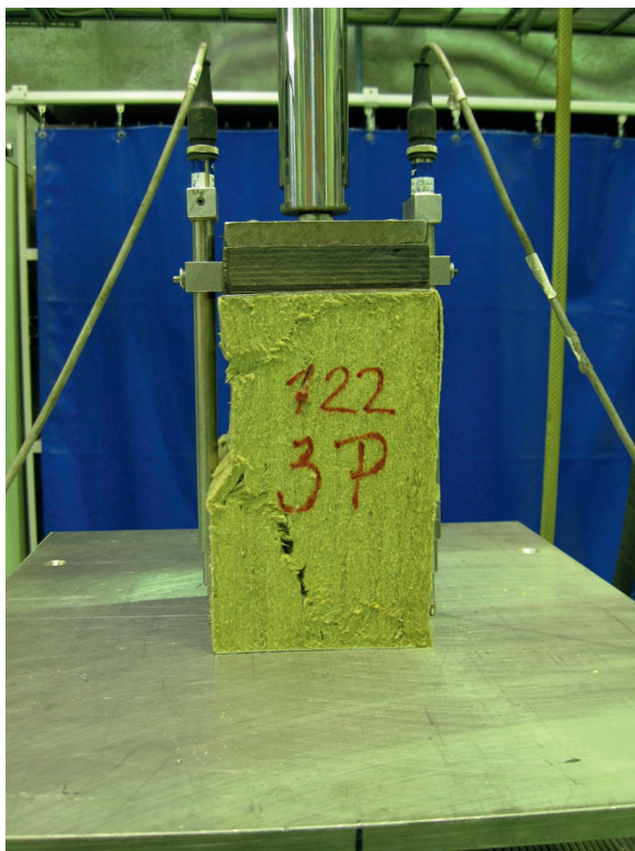
Figure 12: Compression test failed specimen
