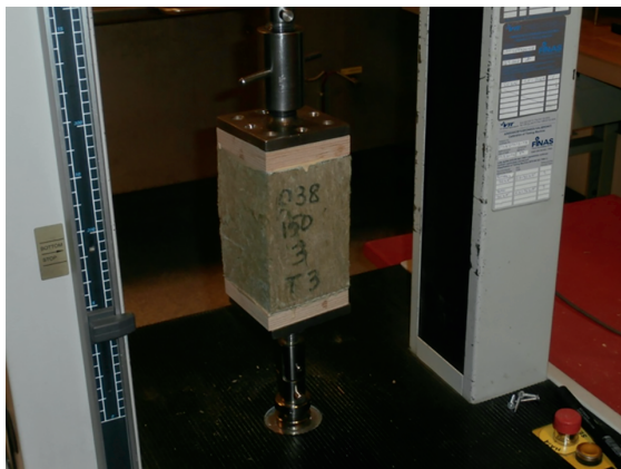
Figure 13: Cross-panel tensile test - measurement of the movement from loading bridge
