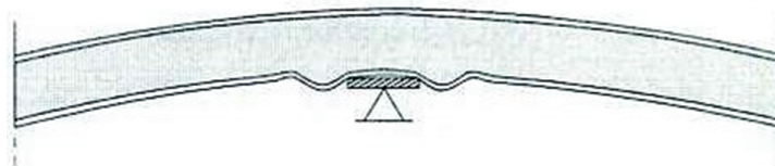
Figure 22: Wrinkling of the face at internal support, under regular loading
